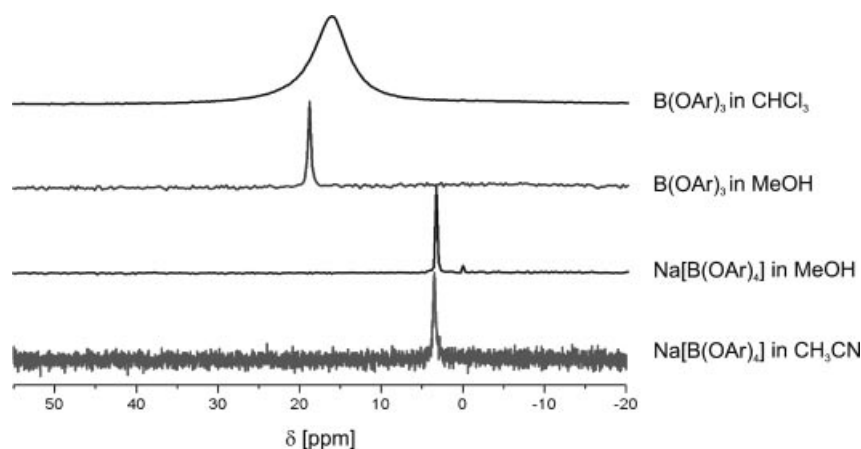
Figure 5. ^{11}\text{B} NMR studies of trigonal and tetragonal boron species (Ar = 2,4-dimethylphenyl).
