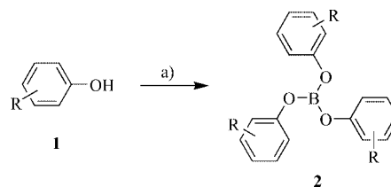
Scheme 1. a) B(OH) 3 , toluene, 12 h reflux with a Dean–Stark trap.
