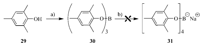
Scheme 3. a) \text{B(OH)}_3 , toluene, 24 h reflux with a Dean–Stark trap; b) 29 , NaH, THF.
