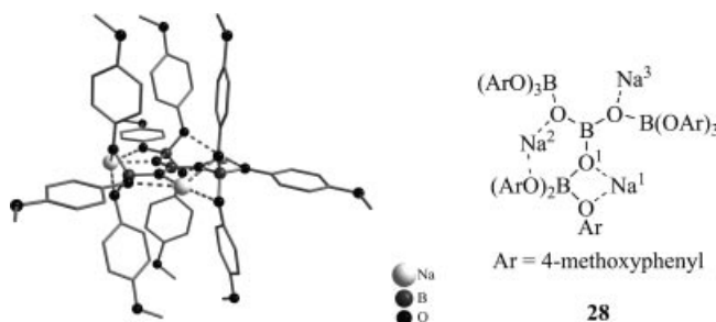
Figure 2. Left: X-ray structure of the tetraborate 28 ; right: coordination pattern.
