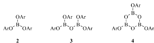
Figure 1. Major products by the condensation reaction of 1 with boric acid.
