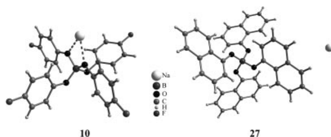
Figure 4. Molecular structures of tetraphenoxyborates 10 and 27 determined by X-ray analysis.
