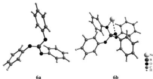
Figure 3. Molecular structure of triphenoxyborane ( 6a ) and the tetraphenoxyborate ( 6b ) determined by X-ray analysis.
