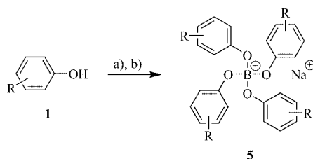
Scheme 2. a) \text{B}(\text{OH})_3 , toluene, 12 h reflux with a Dean–Stark trap; b) Na, 1 , THF, room temp.
